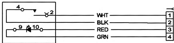
WIRING DIAGRAM
