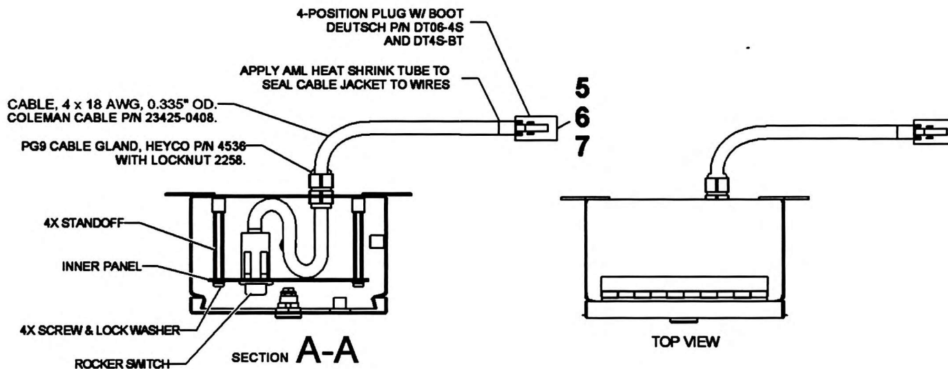
WIRING DIAGRAM
